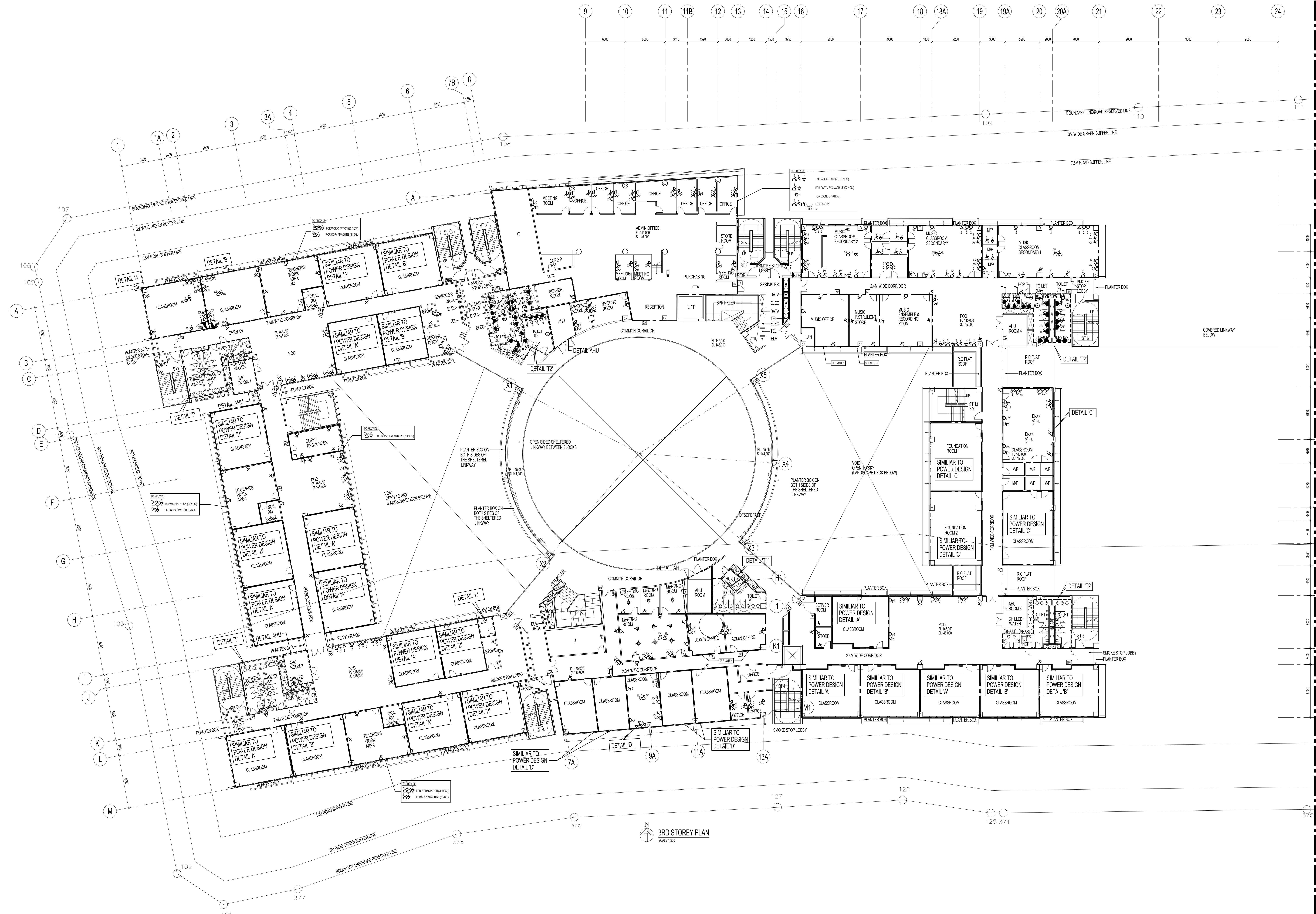
3RD STOREY PLAN (PART A) ACADEMIC BLOCK SCALE 1:200
